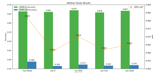
Figure 6: Ablation study results on CIFAR-10, CIFAR-100, and NIPD datasets. The bar charts show the accuracy on CIFAR-10 and CIFAR-100 datasets, while the line plot represents the mAP on the NIPD dataset.
