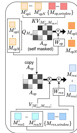
Figure 3: Operation Composition Unit
