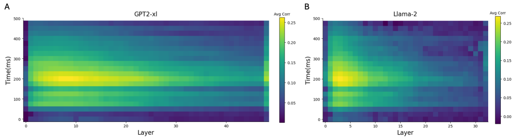
Figure 3: Pearson correlation between actual MEG responses and predicted responses from (A) GPT-2 XL and (B) Llama-2 across LM layers and time after word onset on the Harry Potter dataset. Both models exhibit high correlations in early and intermediate layers at around 200ms. Correlation is computed across words and averaged across MEG channels.
