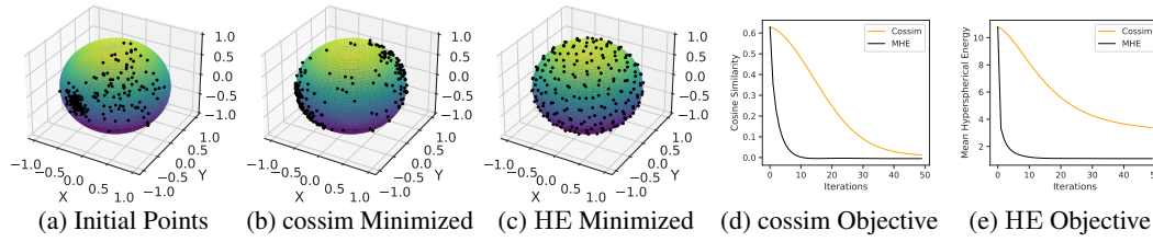
Figure 2: Comparison between optimizing cosine similarity (cossim) or HE on a sphere. (a) initial random set of points placed on sphere. (b-c) the final set of points after 50 iterations either cossim or HE as the similarity metric. (d-e) the value of cossim/HE with respect to the number of iterations. The orange line indicates that cossim is minimized and the black line indicates that HE with s = 2 is minimized. Both methods used gradient descent with a learning rate of 0.75 and momentum 0.9.
