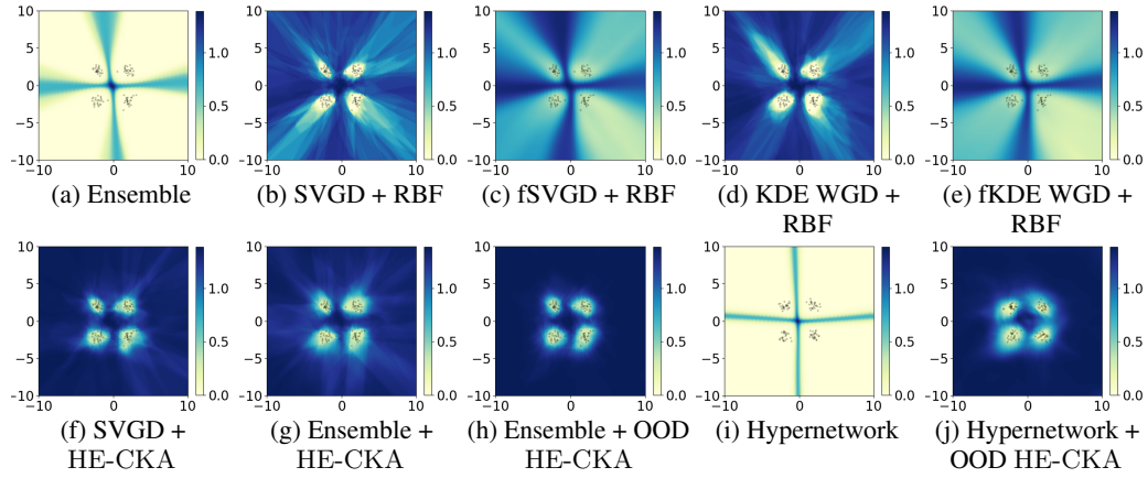
Figure 3: Predictive entropies (PE) on a four-cluster 2D classification task. Darker values indicate higher entropy, lower confidence regions, and lighter values indicate higher confidence regions. (b) and (d) use an RBF kernel on ensemble member weights, whereas (c) and (e) use an RBF kernel on ensemble member outputs. (f) and (g) use the HE-CKA, RBF feature kernel, for feature diversity on inlier points. Both (h) and (j) use HE-CKA and OOD entropy terms. All methods were trained on an ensemble of 30 four layer MLPs for 1k iterations with the same seeds.
