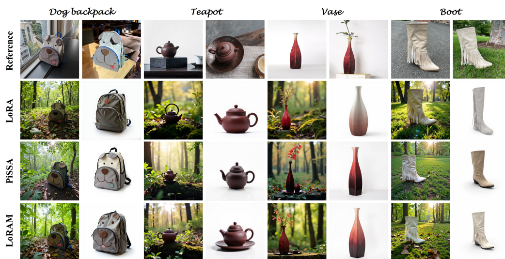
Figure 4: Comparison of LoRA, PiSSA, and LoRAM on image customization task. Experiments conducted with the state-of-the-art FLUX.1-12B model using rank 8.
