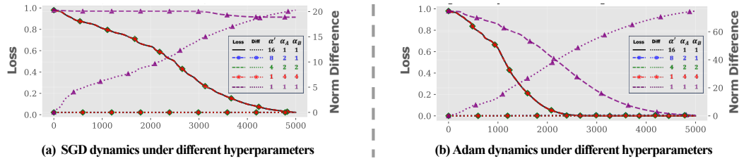
Figure 6: A detailed view of the validation of Proposition 1, separating the SGD and Adam optimization phases. Each curve represents a model with a unique hyperparameter combination. The norm difference (right axis) aggregates the Frobenius norm discrepancies between the baseline model (black curve) and others across all layers. The results show that diverse hyperparameter sets can produce identical optimization trajectories, confirming our theoretical equivalence framework.
