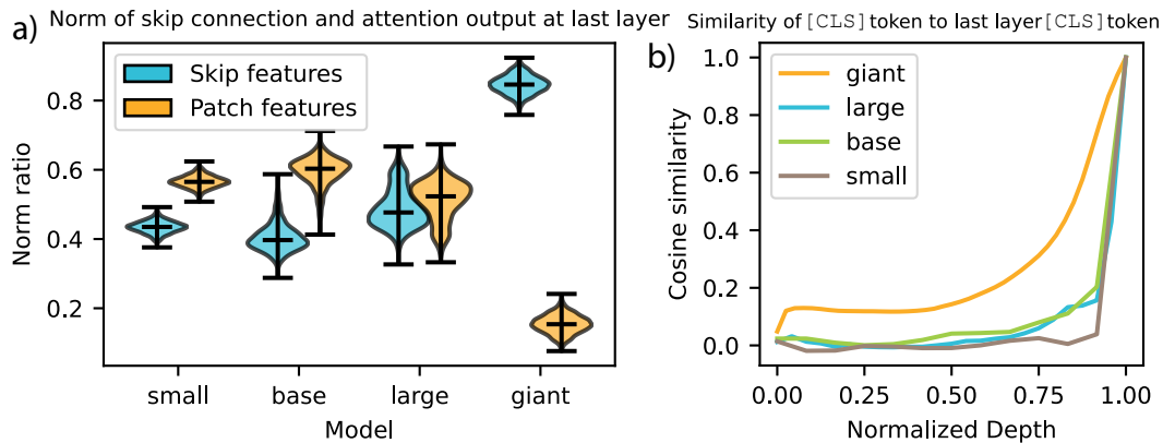
Figure 5: a) After the self-attention mechanism, a skip connection sums the attention output and the hidden states from the previous layer, providing an alternative way for the [CLS] token to attend to itself. Since the attention weights are given only implicitly, we plot the L_2 -norm of the contributions of the skip connections and the patch features to the [CLS] token as a proxy. We observe that in the 'giant' model, the global output is primarily determined by previously computed features, rather than the patch features. b) We show the cosine similarity of the [CLS] token at all model layers to the [CLS] token at the last layer. The three smaller models exhibit a large jump at the very last layer, indicating that the [CLS] token at the last layer is strongly influenced by the patch tokens. Conversely, the [CLS] token of the 'giant' model converges to the final output more smoothly, explaining its low reliance on the patch features at the last layer.
