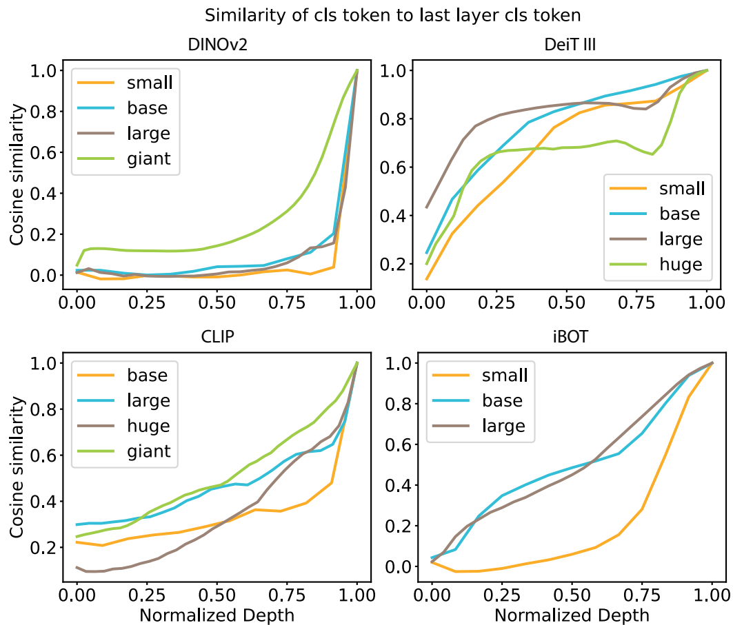
Figure 9: Layerwise similarity between the [CLS] token and the last-layer [CLS] token as discussed in Section 4. CLIP and iBOT mirror the DINOv2 behavior, whereas DeiT III does not exhibit a clear relationship between model size and early [CLS] integration. Note that DeiT III is the only model trained with drop-path regularization, which may explain why all model sizes integrate final output information early in the hierarchy.
