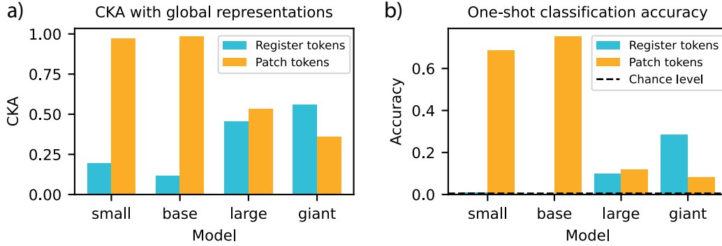
Figure 3: a) Centered kernel alignment between the global [\text{CLS}] token output, and [\text{CLS}] token output computed while only attending to either register tokens or patch tokens. Patch tokens yield a faithful representation of the global output for smaller models, but the connection between local and global features breaks down with increasing model size. b) One-shot classification accuracy on the 1000 Imagenet classes. The classifier is trained on the global [\text{CLS}] output and then tested on output based on patch and register tokens, respectively. Attending only to the patch tokens yields poor performance in the larger models, corroborating the finding that global representations are not formed by attending to the patch features.
