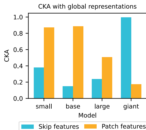
Figure 6: Centered kernel alignment between the standard [CLS] token output, and [CLS] token output computed using either only patch token features or the skip connection features from DINOv2. We observe that the findings from Fig. 5, that the giant model attends primarily to the skip connection, does indeed lead to disconnected representations between global features and patch features. This shows that the skip connection for the [CLS] token can by itself lead to a violation of the patch integration assumption.
