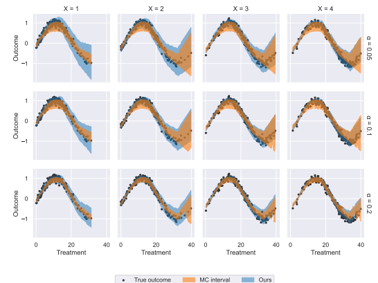
Figure 6: CP intervals for multiple significance levels \alpha for Dataset 1 with intervention \Delta = 5 .
