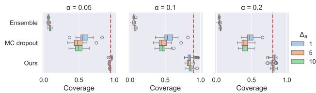
Figure 5: Comparison of faithfulness on dataset 2 across 50 runs. Larger values are better.
