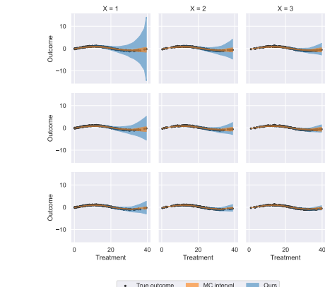
Figure 12: Prediction intervals for multiple significance levels \alpha for the synthetic dataset 2 with intervention \Delta = 10 .
