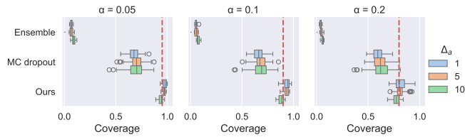
Figure 4: Comparison of faithfulness on dataset 1 across 50 runs. Larger values are better. For each \alpha , the plots show how often the empirical intervals contain the true outcome. Intervals should ideally yield a coverage of 1 - \alpha (red line).
