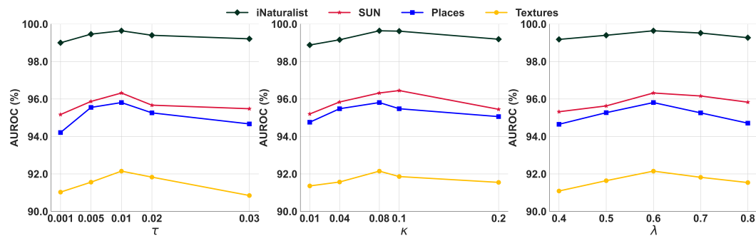
Figure 1: Ablation study on ImageNet-1K w.r.t hyper-parameters \tau (left), \kappa (middle) and \lambda (right)
