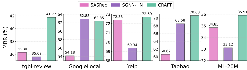
Figure 9: MRR scores of CRAFT, SASRec and SGNN-HN on unseen-dominant bipartite datasets.
