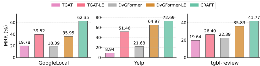
Figure 6: Evaluating the impact of learnable node embeddings and cross-attention: CRAFT vs. TGAT/DyGFormer with and without learnable embeddings (LE).
