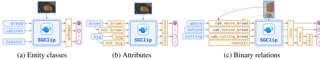
Figure 3: Illustration of the inference modes of SGClip for three types of concepts: entity classes, attributes, and binary relations. While the model stays the same, the three inference modes perform different pre- and post-processing for a more accurate semantic estimation of probabilities.
