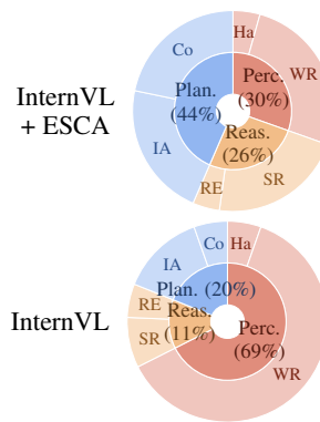
Figure 7: Error decomposition 1 of InternVL with or without ESCA, manually inspected on 60 EB-Navigation tasks.
