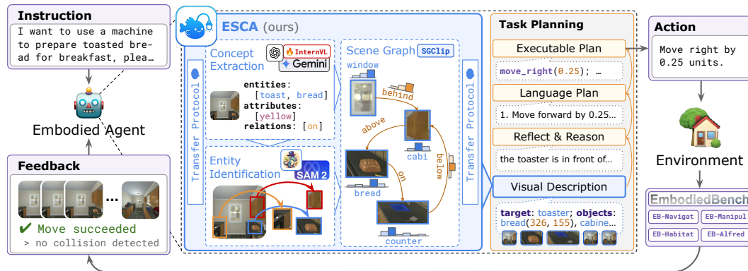
Figure 1: An overview of embodied agent pipeline augmented with ESCA. In each cycle, the agent takes in an instruction and the environmental feedback and outputs a concrete executable action, through a sequence of perception, reasoning, and planning. The action is then executed and the environment will provide the next state. Notably, ESCA contextualizes the task planner with grounded visual features represented as a scene graph.
