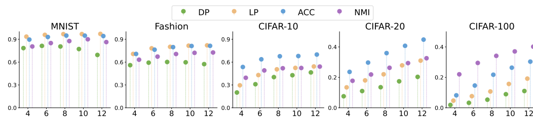
Figure 3: Hierarchical clustering performance on all evaluated datasets at varying depth of \mathcal{T} . X-axis: depth, Y-axis: performance.
