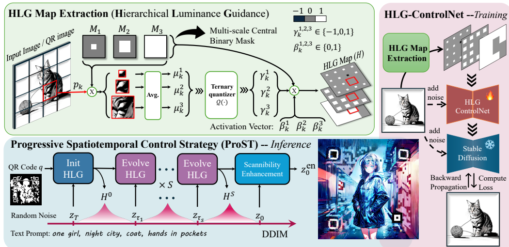
Figure 2: Illustration of the proposed AnimateQR framework. The green box depicts the extraction of the Hierarchical Luminance Guidance (HLG) map from input images. The red box outlines the training of the HLG-ControlNet, while the blue box highlights the inference stage using the proposed Progressive Spatiotemporal control (ProST) strategy. During training, we extract HLG map with randomly sampled activation vector \beta_k as detailed in Section 3.3. During inference, animated QR codes are generated via the DDIM process using a Stable Diffusion model equipped with HLG-ControlNet (as the control unit) and AnimateDiff (as the motion module). The HLG map is progressively updated by the Evolve HLG module as detailed in Section 3.4, enabling adaptive spatiotemporal control throughout the denoising process.
