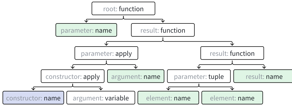
Figure 7: An example AST of f :: \text{Int} \rightarrow \text{Either } a \text{ Char} \rightarrow (\text{Int}, \text{Char}) \rightarrow \text{Float} .
