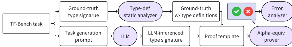
Figure 3: Pipeline to evaluate LLMs on TF-Bench.
