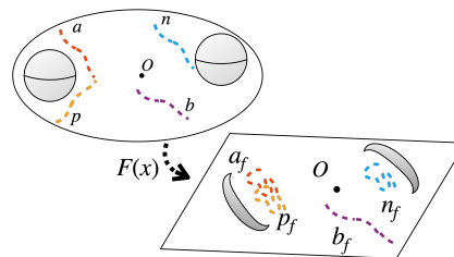
Figure 1: Mapping input data (left) to learned feature space (right); Training classes are solid balls, unseen classes a, b, p, n are dashed lines. Cohesion : Strong Cohesion occurs for a, p, n , which have high similarity to the training data compared to b . Separability of a, n : assigned to different training class, they show high Separability . Separability of a, p : assigned to the same training class, they exhibit low Separability .
