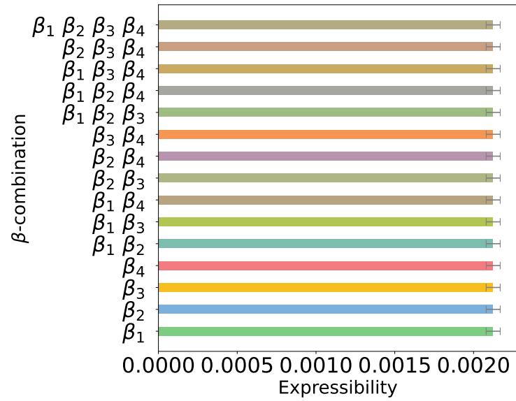
(a) F_{0,L}
