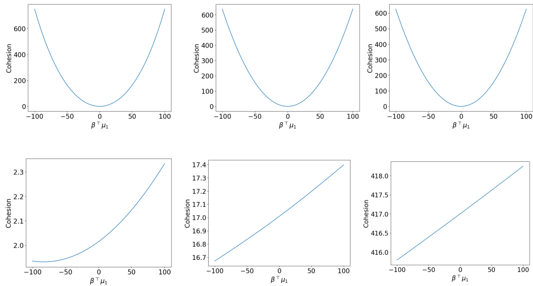
Figure 11: Component analysis of Cohesion in \mathbb{R}^{2000} , \mathbb{R}^{20000} , \mathbb{R}^{320000} (left to right) in the range [-100, 100] . Top: Cohesion of the dominant component s_L i.e. Equation (6). Bottom: sum of the other terms in Equation (67), which make only suppressed contributions.
