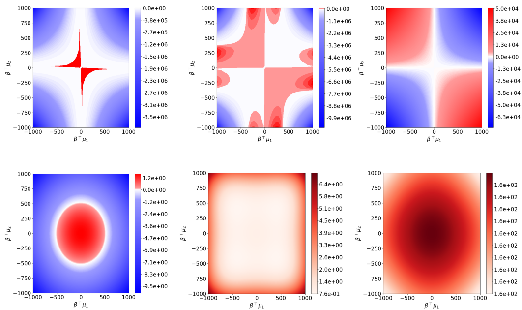
Figure 16: Component analysis of Separability in \mathbb{R}^{2000} , \mathbb{R}^{20000} , \mathbb{R}^{320000} (left to right) in the range [-1000, 1000] . Top: Separability of the dominant component s_L i.e. Equation (7). Bottom: sum of the other terms in Equation (68), which make only suppressed contributions.
