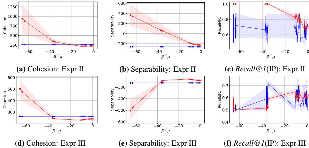
Figure 4: Upper row: In Expr II, all metrics increase as |\beta^T \mu| increases. Lower row: In Expr III, where two test classes are assigned to a single train class, Recall@1 and Separability tend to decrease as |\beta^T \mu| increases. This aligns with our predictions. In all cases, results using Data 1 are reported. The red line — represents the values after one step of training, i.e., F . The blue line — represents the values from initialization, i.e., F_0 .
