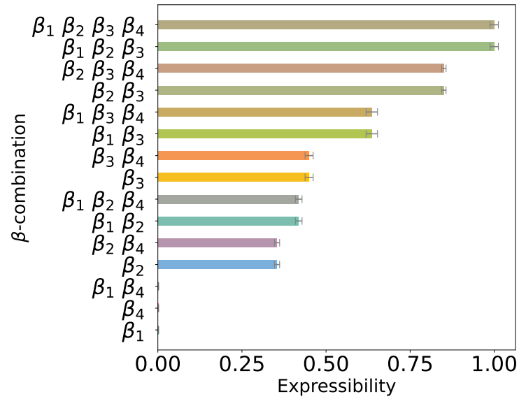
(a) Theory
