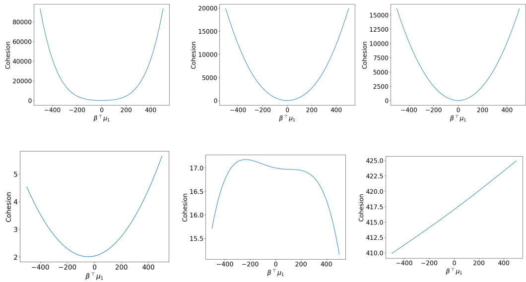
Figure 12: Component analysis of Cohesion in \mathbb{R}^{2000} , \mathbb{R}^{20000} , \mathbb{R}^{320000} (left to right) in the range [-500, 500] . Top: Cohesion of the dominant component s_L i.e. Equation (6). Bottom: sum of the other terms in Equation (67), which make only suppressed contributions.
