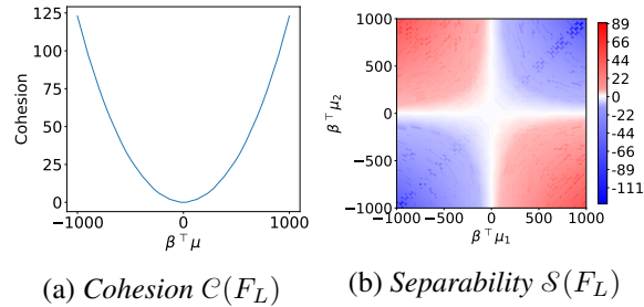
Figure 2: \mathcal{F} by adjusting \beta^\top \mu_1 and \beta^\top \mu_2 . We set n = 320000 , \mu_1 = -\mu_2 \in \mathbb{R}^n and \|\mu_1\|, \|\mu_2\|, \|\beta\| = 1 .
