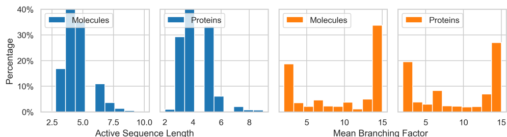
Figure 4: Constrained generation space structure analysis: Distribution of active sequence lengths for molecules and proteins (left), and mean branching factors for molecules and proteins (right). Active sequence length represents the number of positions requiring actual prediction decisions, while branching factor indicates the number of valid token choices at each active position.
