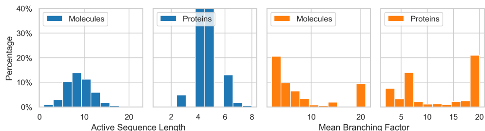
Figure 5: Active sequence lengths and branching factors for BioSNAP dataset with raw representations.
