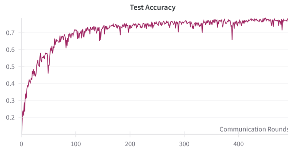
Figure 8: Test Accuracy
