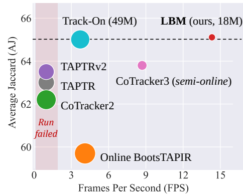
Figure 2: Efficiency comparison on TAP-Vid DAVIS benchmark with an NVIDIA Jetson Orin NX super. LBM shows efficiency with higher inference speed and smaller model size. The size of the circles corresponds to the number of parameters.
