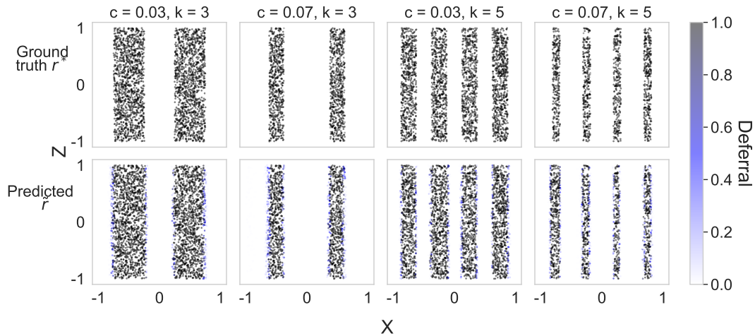
Figure 2: Top ) Ground truth decision boundary \hat{r}^*(x) with 2 costs values c = 0.03, 0.07 and number of classes K = 3, 5 . Bottom ) Learned \tilde{r}(x) of the model that was trained with our surrogate loss. In all cases, the two decision boundaries are perfectly aligned, confirming our result that the model trained with the proposed surrogate loss successfully learns the optimal decision function. As the cost increases, the black region which represents points deferred to f_2 shrinks.
