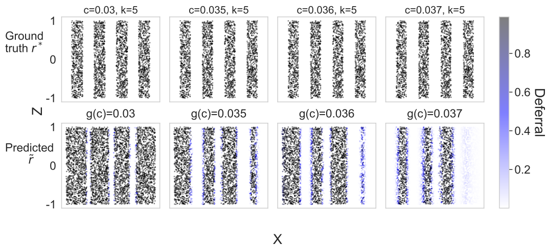
Figure 3: Top ) Ground truth decision boundary \hat{r}^*(x) with 4 costs values and number of classes K = 5 . Bottom ) Learned \tilde{r}(x) of a model trained with the additive cross-entropy surrogate loss with g(c) = c , for varying c values. Unlike the model trained with the hinge-based surrogate, the learned decision patterns are generally wrong and not consistent.
