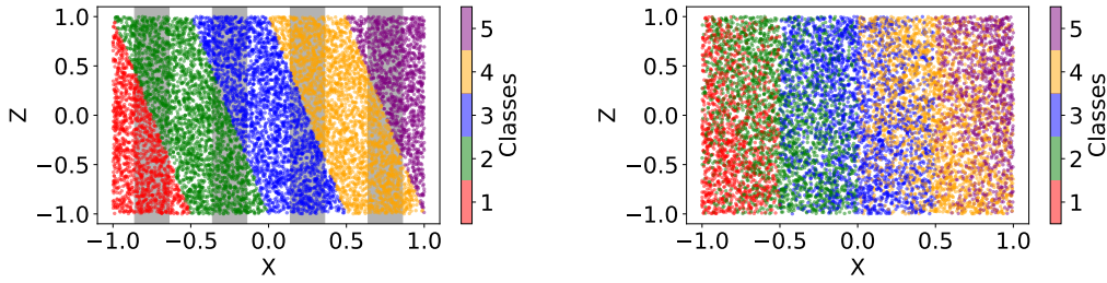
Figure 1: Visualization of multi class synthetic dataset with k = 5 . Left) Max probability labels \arg \max_y p(Y = y|X, Z) . The black shaded region indicates where the optimal decision rule is to defer to f_2 ( r^*(x) = 1 ), given a cost of c = 0.03 . Right) Samples x, z, y \sim p(X, Z, Y) of the synthetic experiment.
