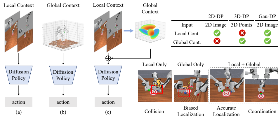
Figure 1: Both local and global context are essential in multi-agent collaboration. Comparison of multi-agent decision-making using different types of contextual information. (a) Using only local context leads to miscoordination such as collisions due to lack of global awareness. (b) Using only global context provides a holistic scene view but lacks detailed local features, resulting in inaccurate control, such as biased localization. (c) Our proposed method, GauDP , fuses global context, which is reconstructed from 2D local images via a shared 3D Gaussian representation, on top of local observations. This integration enables both accurate localization and coordinated execution. Our proposed method, based solely on 2D observations, effectively aggregates global context on top of the local context.
