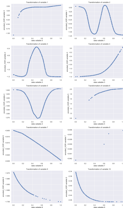
Figure 37: Illustration of the graphical analysis of the transformations: on a bivariate setting
