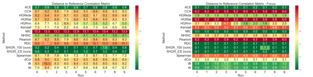
(c) Heatmap of distances to Reference Correlation ( d_{CM_{ref}} ) (d) Heatmap of distances to Reference Correlation - focus ( d_{CM_{refFocus}} )
