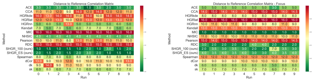
(e) Heatmap of ranks of distances to Reference Correlation ( d_{CM_{ref}} ) (f) heatmap of ranks of distances to Reference Correlation - focus ( d_{CM_{refFocus}} )
