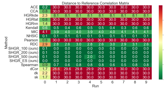
(b) Heatmap of distance to Reference Correlation Matrix
