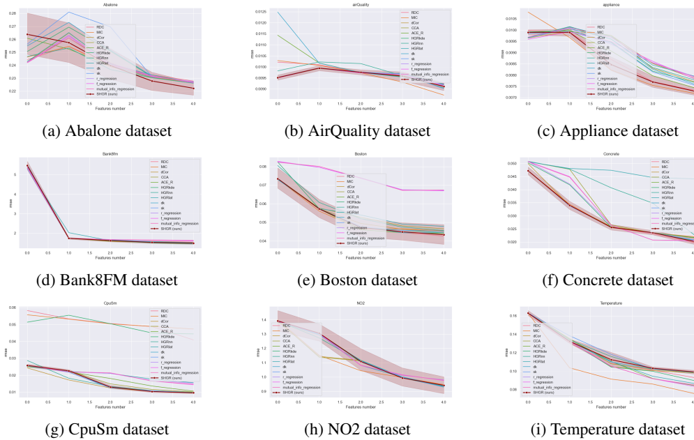
Figure 38: Feature selection on real-world datasets with SHGR shown in red (lower is better): based on maximal correlation (bivariate correlation)
