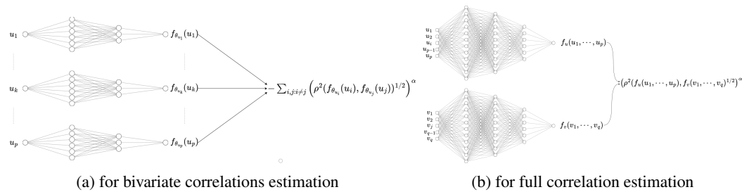
Figure 1: Cross-Encoder Architecture
