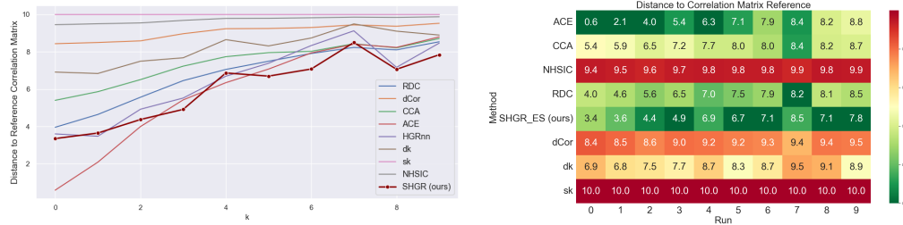
Figure 19: Robustness to noise: distance to Reference Correlation Matrix (lower is better) ; results for multivariate correlations
