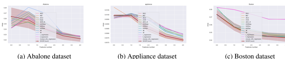
Figure 7: RMSE for test set prediction with feature selection on real-world datasets (lower is better); Based on maximal (bivariate) correlation - Results with SHGR are red
