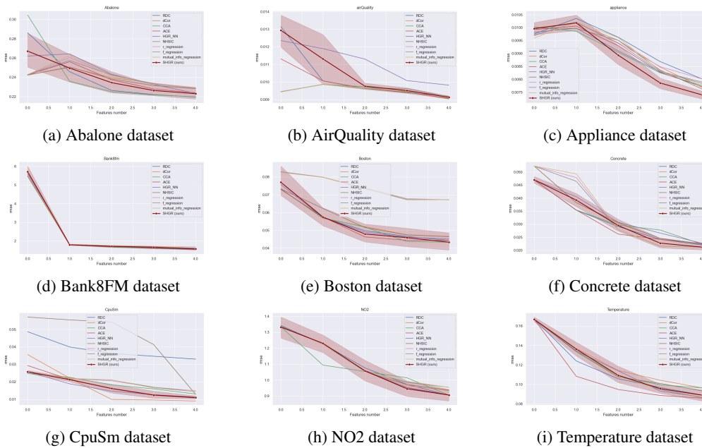
Figure 39: Feature selection on real-world datasets with SHGR shown in red (lower is better): based on maximal correlation contribution (multivariate correlation)
