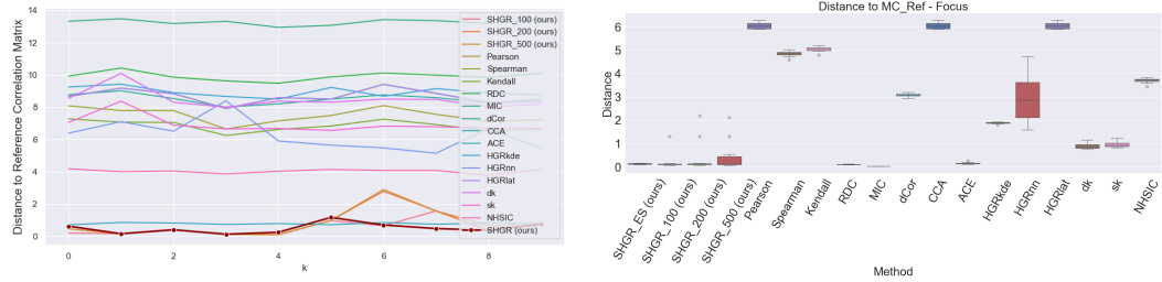
(a) Lineplot of distances to Reference Correlation ( d_{CM_{ref}} ) (b) Boxplots of distances to Reference Correlation - focus ( d_{CM_{refFocus}} )
