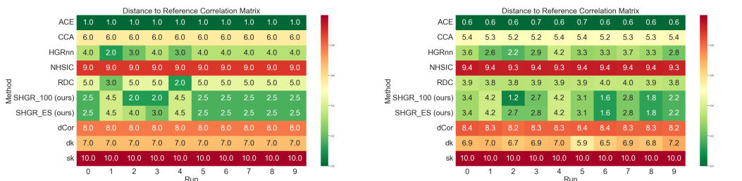
(a) Heatmap of ranks of distances to Reference Correlation ( d_{CM_{ref}} ) (b) Heatmap of distances to Reference Correlation ( d_{CM_{ref}} )
