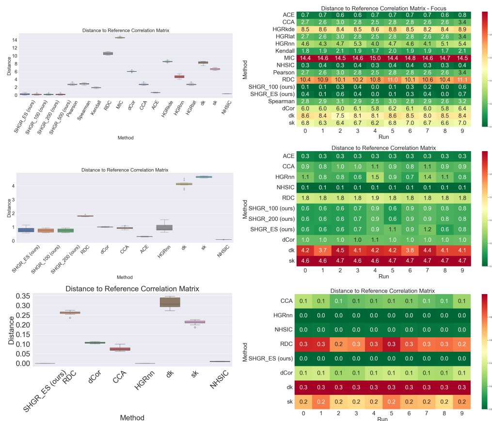
Figure 20: Robustness to hallucination: distance to Reference Correlation Matrix (lower is better) ; for bivariate correlations (up), multivariate correlations and full correlations (down)
