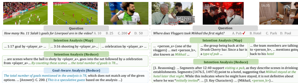
Figure 7: Case Analysis. (Left) Recalling the motivating example (Fig. 1), MR. Video checks every scene in detail (Map) and aggregates the whole video (Reduce). Although it misses some goals due to strict criteria (shooting, goal, and celebration), MR. Video shows the desired behavior of counting exhaustively . (Right) This example demonstrates how a consistent character name (Mikhail) benefits the reasoning process of MR. Video (first night).
