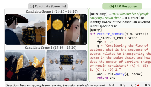
Figure 5: Customized Queries for Perception. With this question requiring detailed visual perception, MR. Video proposes goal-aware queries for the VLMs, confirming the criteria.
