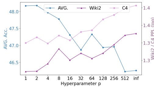
Figure 7: Effect of p in heuristic merge ratio. As p grows, more parameters from layers with higher BI scores are merged.
