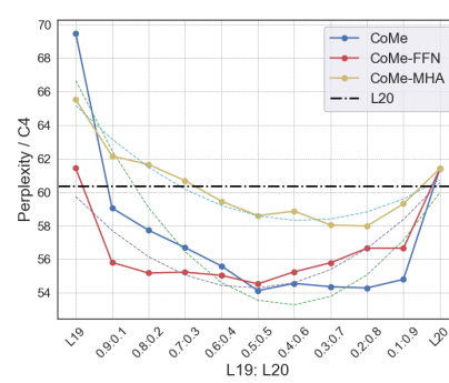
Figure 14: Merge adjacent layers with CoMe at different ratios, using the C4 calibration dataset.
