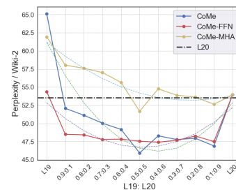
Figure 11: Merge layers with CoMe. The setting is the same as Fig. 3.
