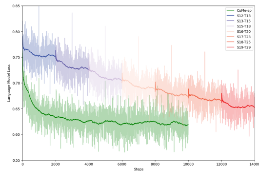
Figure 12: Cross Entropy loss curves for using CoMe-mp and CoMe-sp during post-training. The loss curves for multiple subprocesses of CoMe-mp are concatenated in the order of training.
