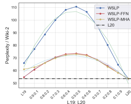
Figure 3: Merge adjacent layers with linear weight aggregation. First, we reduce LLaMA-2-7b’s layer number to 23 with ShortGPT. Second, the components in layers 19 and 20 are merged at different ratios. When merging MHA or FFN, the other component is retained from layer 20.
