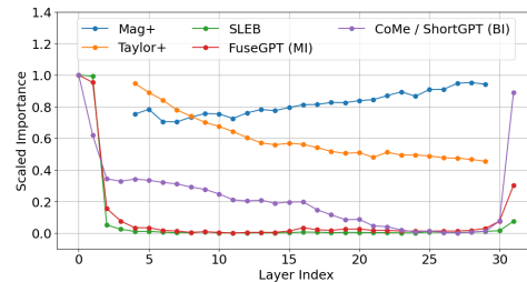
Figure 2: Comparative analysis of normalized layer importance score across different methods. The score of SLEB and FuseGPT is derived from the first-round pruning.
