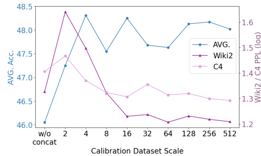
Figure 10: Effect of calibration data scale. CoMe achieves optimal performance with samples more than 128.
