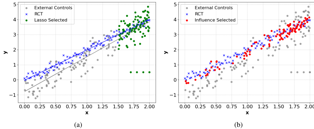
Figure 1: Borrowing behavior comparison of different approaches in a synthetic example. (a) The borrowed samples of the adaptive lasso-based borrowing approach [17]. (b) The borrowed samples of the proposed influence-based borrowing approach. The influence-based approach identifies a set of samples with highly comparable. Details of the synthetic example can be found in Section 7.
