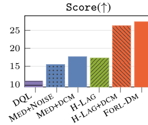
Figure 8: DM Ablations
