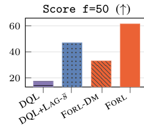
Figure 10: Intra-Episode Performance
