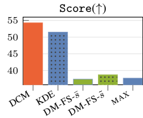
Figure 9: Candidate Selection
