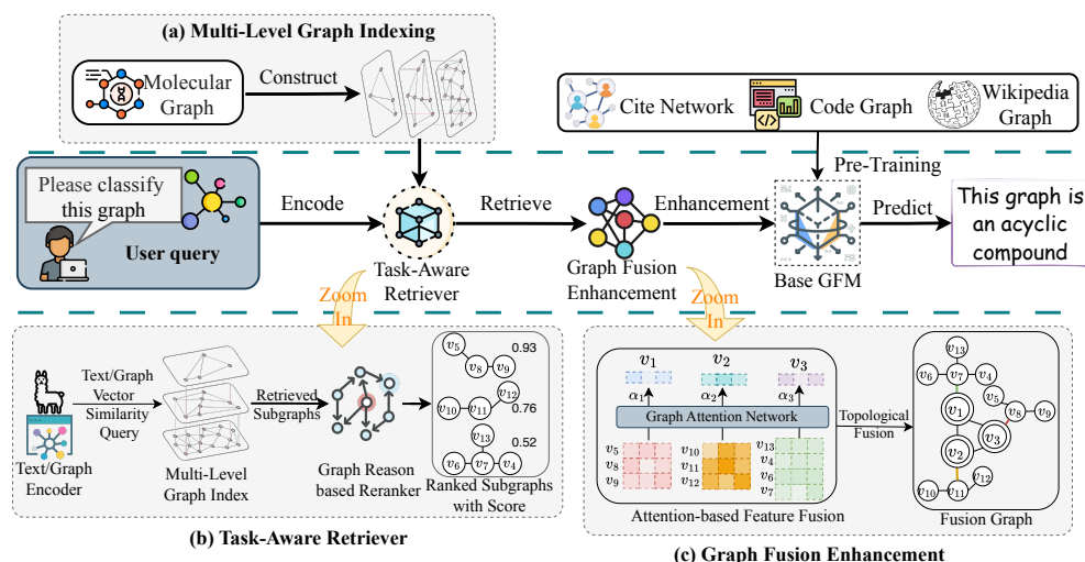
Figure 2: The overall architecture of RAG4GFM . RAG4GFM dynamically augments a Base GFM by: (a) constructing a “Multi-Level Graph Index” (b) retrieving and reranking task-relevant subgraphs based on the user query via a “Task-Aware Retriever”; and (c) fusing the retrieved subgraphs with query information through the “Graph Fusion Enhancement module”, before generation.
