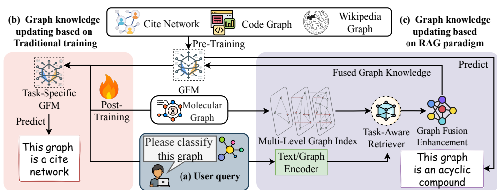
Figure 1: Comparison between conventional training-driven GFM (b) and RAG4GFM (c). (a) A user query comprising a natural-language description and a graph; (b) Conventional GFM relies on task-specific post-training to integrate new knowledge, incurring substantial computational cost; (c) RAG4GFM integrates external graph knowledge at inference time via retrieval and fusion, ensuring faithful reasoning without additional post-training.
