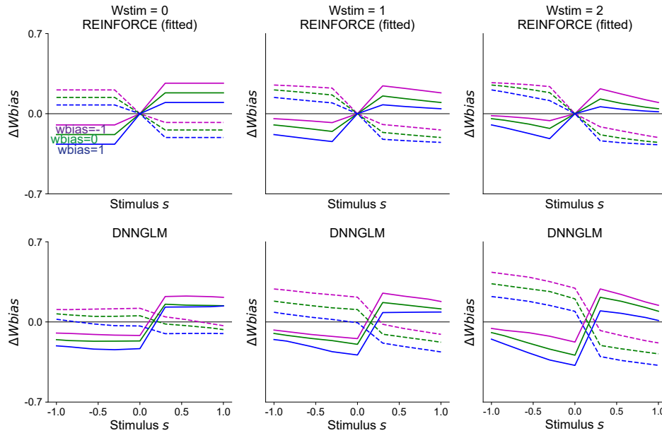
Figure 8: Bias weight update function closely resembles REINFORCE. Similar to Fig. 5, which visualizes the stimulus weight update function, we plot here the inferred update function for the bias weight. We plot REINFORCE (fitted on the DNNGLM) in the top row and DNNGLM on the bottom row. The fitted neural network model captures key qualitative features of the REINFORCE update rule for the bias weight.
