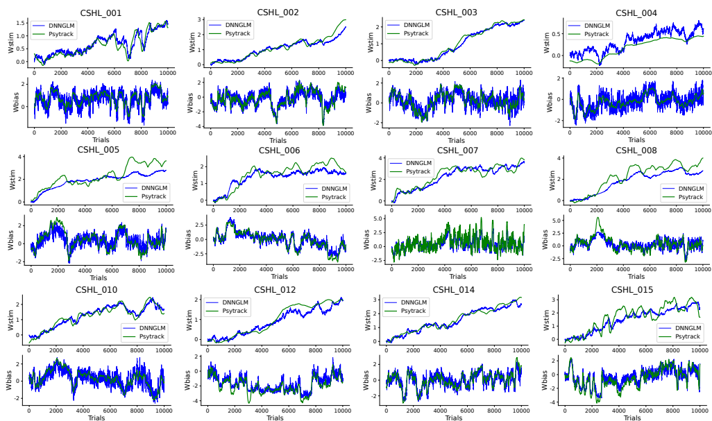
Figure 15: Extended version of Fig. 4A, showing both stimulus and bias weight trajectories across more animals. The decision weights recovered by DNNGLM closely resemble those inferred by PsyTrack.
