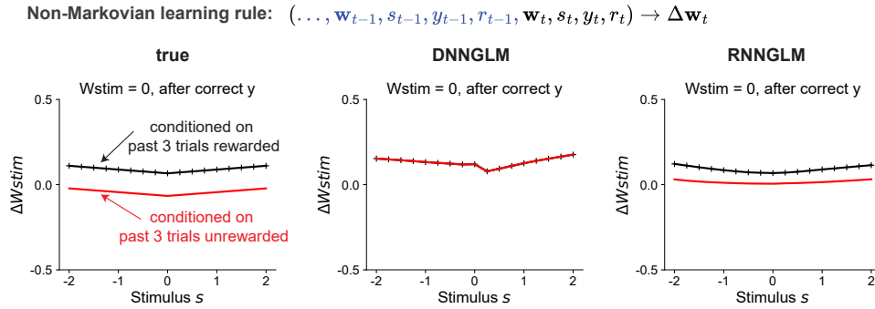
Figure 3: Simulated example with a non-Markovian learning rule. The RNNGLM recovered the reward history dependence present in the ground truth: larger weight updates occur when the past 3 trials were rewarded (black) versus unrewarded (red). Such differences were absent in DNNGLM, as it can only account for Markovian learning rules, where weight updates depend on current trial information. The ability of RNNGLM to capture these effects reflects its greater flexibility. Minor deviations from the ground truth are likely due to finite data effects (Fig. 2C). To keep the figure simple, we only plotted with the learning rule given stimulus weight w_{stim} = 0 and after correct choices, but we observed similar phenomena for other parameter settings.
