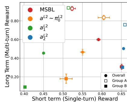
Figure 8: Long-term (multi-turn) vs short-term (single-turn) rewards for all users (overall) and for each user group.
