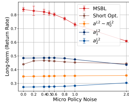
Figure 13: Long term return rate with varying noise \sigma_s in micro policy varies in \{0.0, 0.2, 0.4, 0.6, 0.8, 1.0, 2.0\} .
