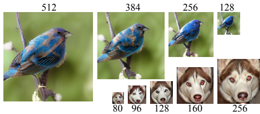
Figure 4: Generated samples from 80px to 512px. FlexVAR demonstrates strong consistency across various scales and can generate 512px images, despite the model being trained only on images \leq 256 px.
