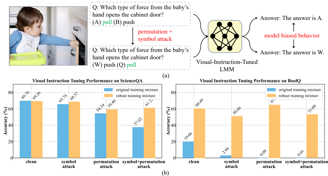
Figure 1: (a) Illustration of biased behaviors exhibited by LMMs. (b) Robustness of visual-instruction-tuned LLaVA-1.5-7B on a multimodal task (left) and LLaVA-1.5-13B on a pure-text task (right) under symbol and permutation attacks. The results highlight a significant decline in accuracy due to underlying dataset biases, and catastrophic forgetting further amplifies the vulnerability. Our curated robust training mixture enhances the model's robustness.
