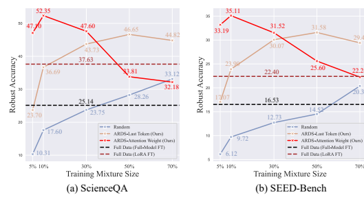
Figure 3: Robust Accuracies (↑) across different sizes of training mixture used for visual instruction tuning of LLaVA-1.5 on ScienceQA and SEED-Bench benchmarks. Robustness is evaluated through incorporating symbol and adversarial permutation attacks.
