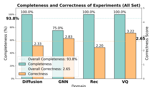
Figure 4: Quantifying Implementation Quality in terms of Completeness and Correctness.
