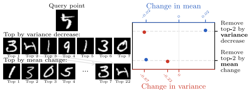
Figure 11: d-TDA for MNIST. d-TDA with influence functions (see Section 4) successfully determines which training examples to remove for a decrease in measurement variance. These differ to examples identified for a change in mean. Different d-TDA variants capture diverse information about the training data. This experiment uses a multi-layer perceptron (MLP) trained on MNIST.
