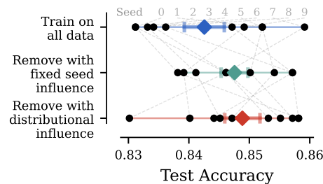
Figure 6: d-TDA > fixed-seed TDA. Test accuracy improvements on CIFAR-10 with a SWIN Vision Transformer from IF data pruning. We compare two approaches to subset selection: 1) traditional TDA with a fixed seed , where for each random seed we remove 5000 datapoints that are predicted to decrease the validation loss the most for the model trained with that specific fixed seed; and 2) distributional-TDA , where for each model we remove 5000 datapoints predicted to decrease the validation loss the most on average. Both methods lead to test accuracy improvements upon the baseline trained with all data. However, d-TDA leads to greater overall improvements on average. Black dots show accuracies for individual models (with seeds indicated in gray), whereas coloured diamonds indicate the average result for each method.
