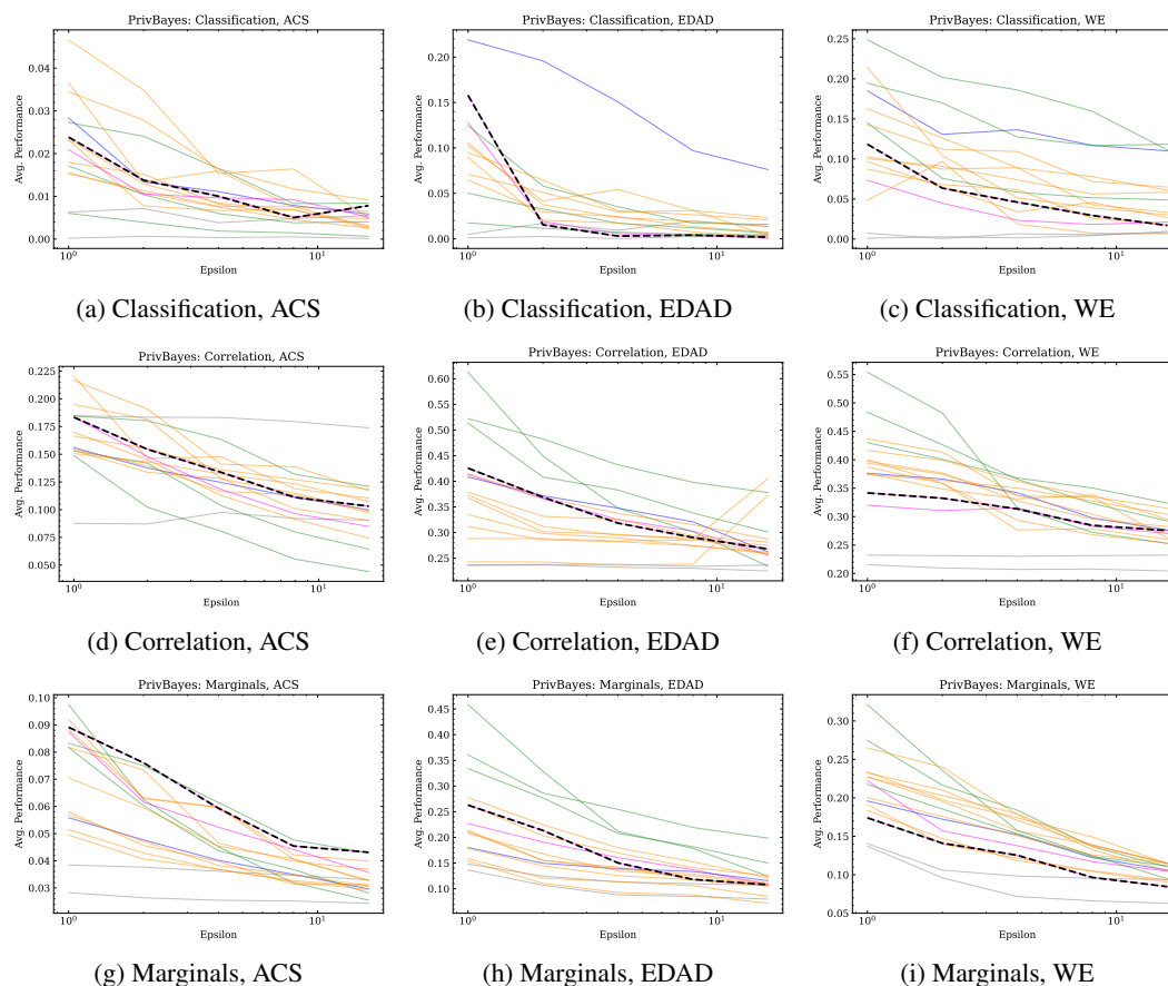
Figure 28: To provide intuition for exactly what the \ell_1 and \ell_2 scores in Figures 26 and 27 attempt to capture, we plot the average performance across epsilon that constitutes each vector, relative to the true performance of the sensitive data (which, in these plots, is the black dotted line). Ideally, for privacy/utility estimation, any public data (surrogate or otherwise) would match the performance of the private data across privacy loss budget parameters. This would allow a practitioner to, say, choose the correct \epsilon based on a performance threshold in absolute terms. Clearly, given the noisiness of the lines (which generally cluster around, but inconsistently track, the black dotted line for private data performance), this is a difficult estimation problem.
