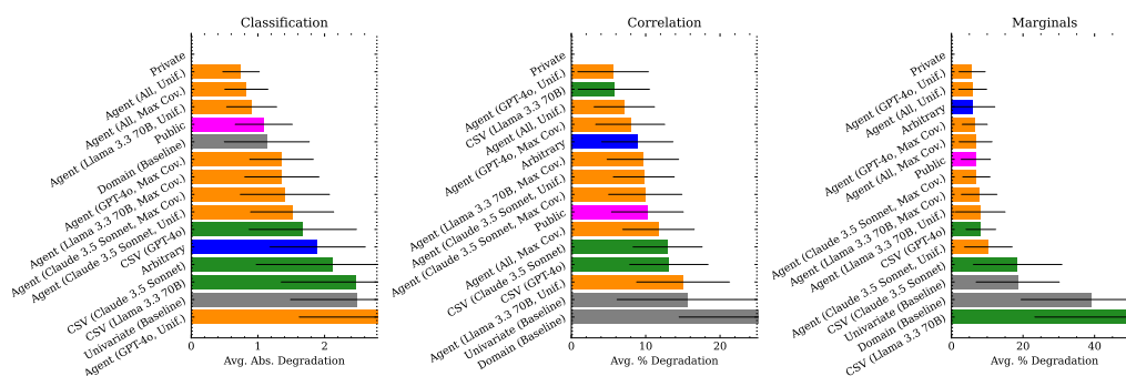
Figure 25: Granular hyperparameter tuning results for WE on the GEM synthesizer. The trends mirror those in ACS, with the Arbitrary baseline maintaining strong performance and Agent-based methods showing similar competitiveness.
