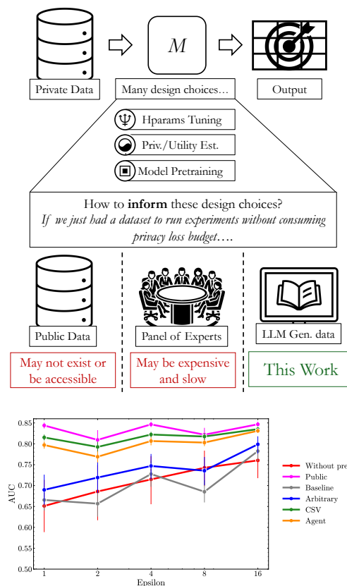
Figure 1: (Top) The premise of this work: Can we utilize LLMs to generate surrogate public data to solve DP auxiliary tasks? (Bottom) The answer is yes ; for example, pretraining on surrogate public data generated through various LLM based methods (green, orange) nearly matches the performance of pretraining on regular public data (magenta), and outperforms no pretraining (red), or pretraining on baselines (gray, blue). Results on the EDAD dataset.
