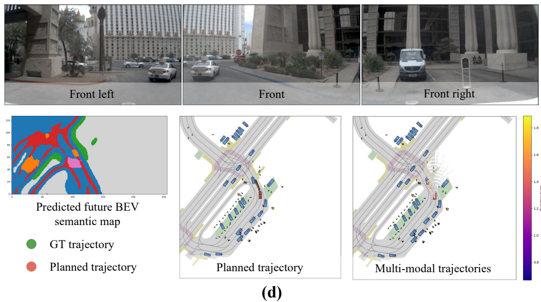
Figure 5: Qualitative results 2 on the NAVSIM dataset. The visualization includes three front-facing camera views: front left, front, and front right, as well as model outputs including the predicted future BEV semantic map, the planned trajectory, and multi-modal predicted trajectories.
