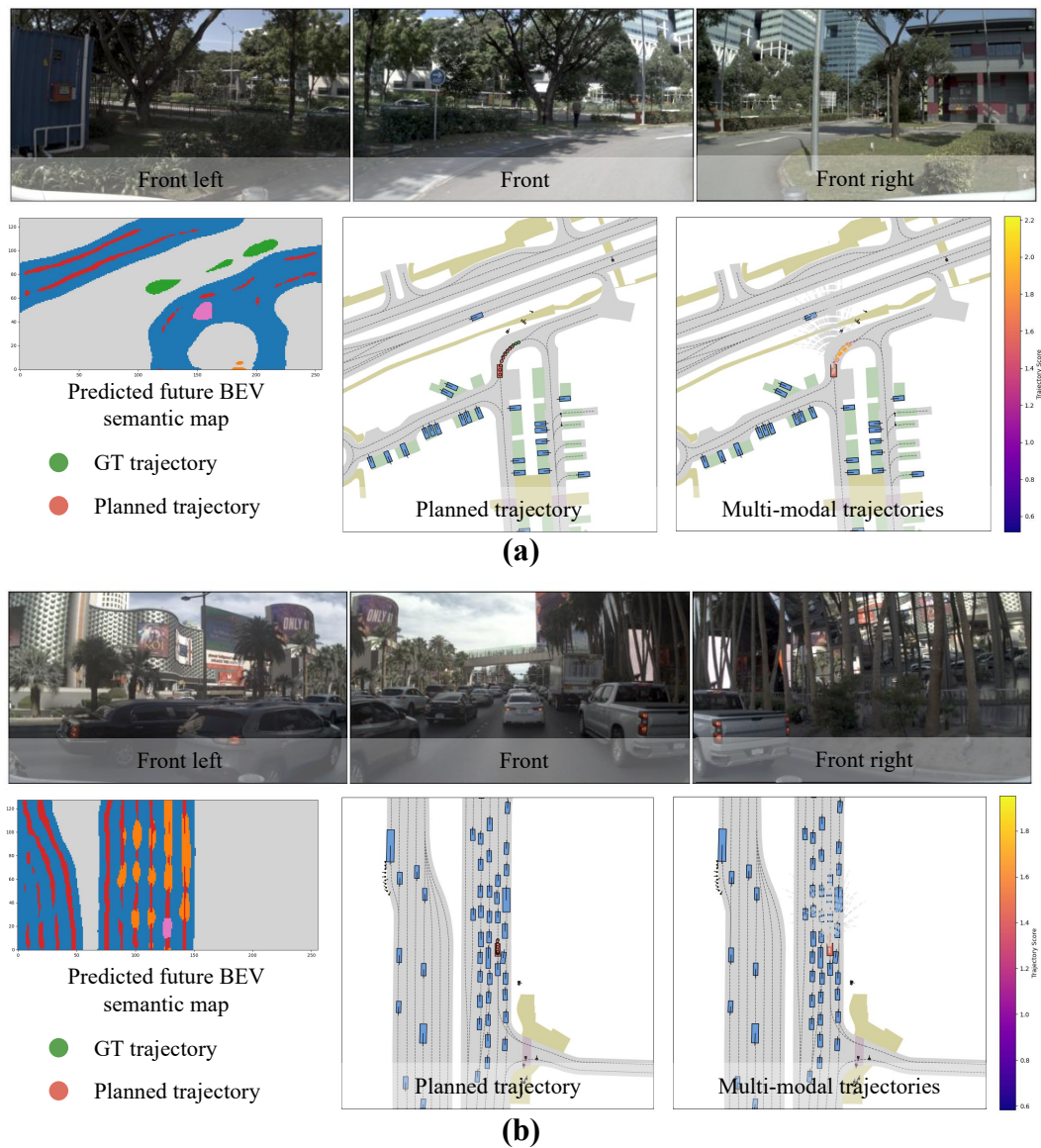
Figure 4: Qualitative results 1 on the NAVSIM dataset. The visualization includes three front-facing camera views: front left, front, and front right, as well as model outputs including the predicted future BEV semantic map, the planned trajectory, and multi-modal predicted trajectories.
