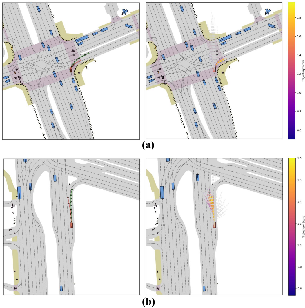
Figure 6: Failure cases from the NAVSIM dataset. In the left figure, the ground-truth trajectory is shown in green , while the top-ranked planning trajectory, selected based on the classification score, is displayed in orange . The right figure illustrates the predicted multi-modal trajectories.
