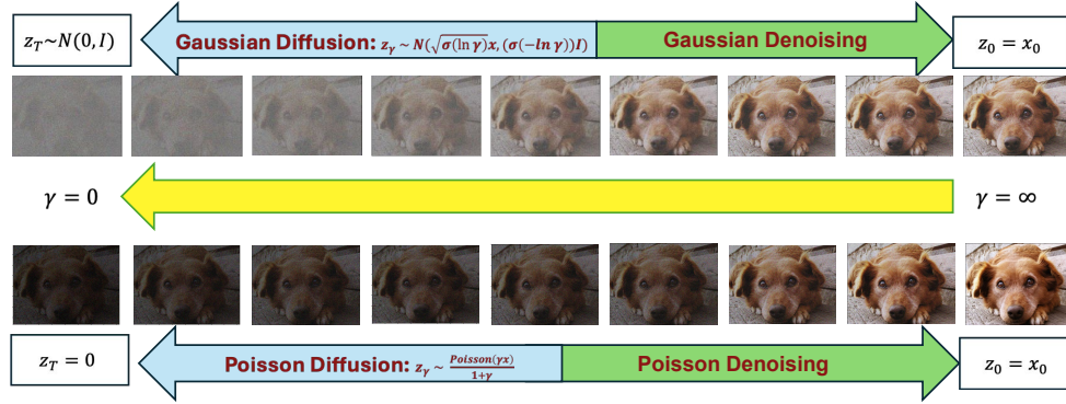
Figure 4: Comparison of Gaussian (top) and Poisson diffusion processes (bottom).
