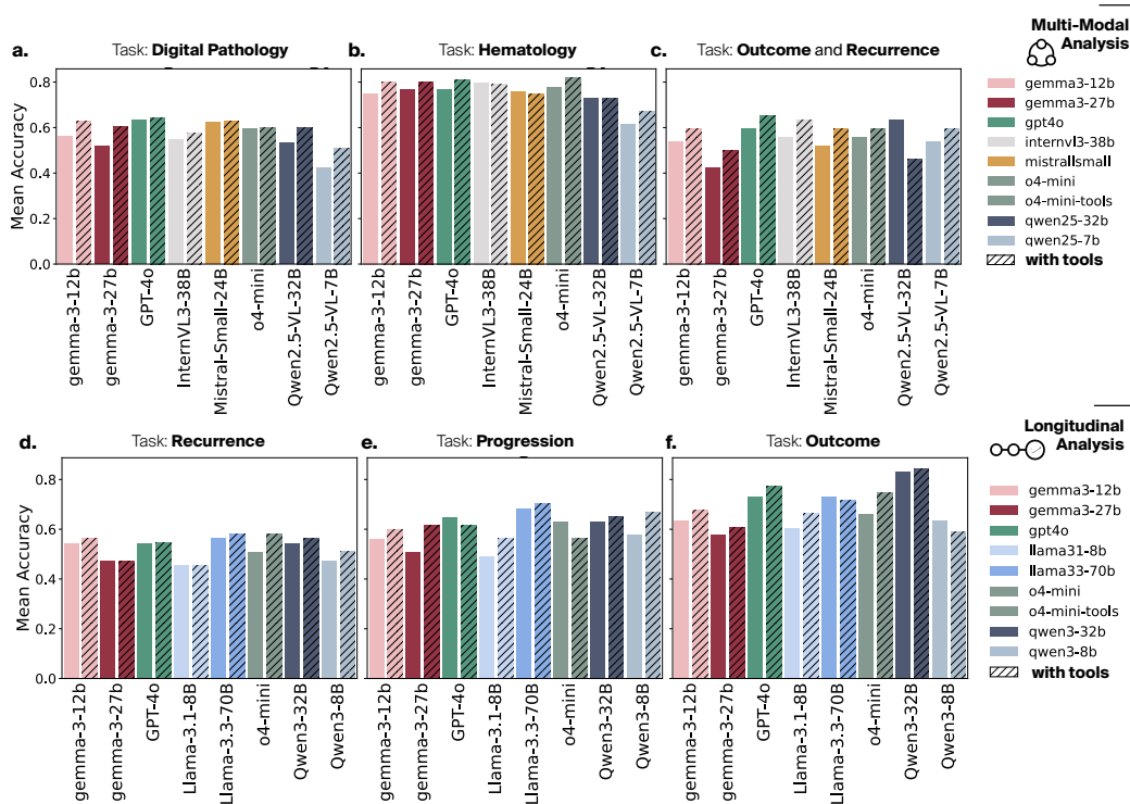
Figure 3: Accuracy across models and tasks for naive and tool-augmented agents. For multi-modal (a–c.) and longitudinal (d–f.) evaluation. Models equipped with tool access (hatched bars) generally show improved accuracy, highlighting the benefit of querying external resources in both multi-modal and temporal settings.
