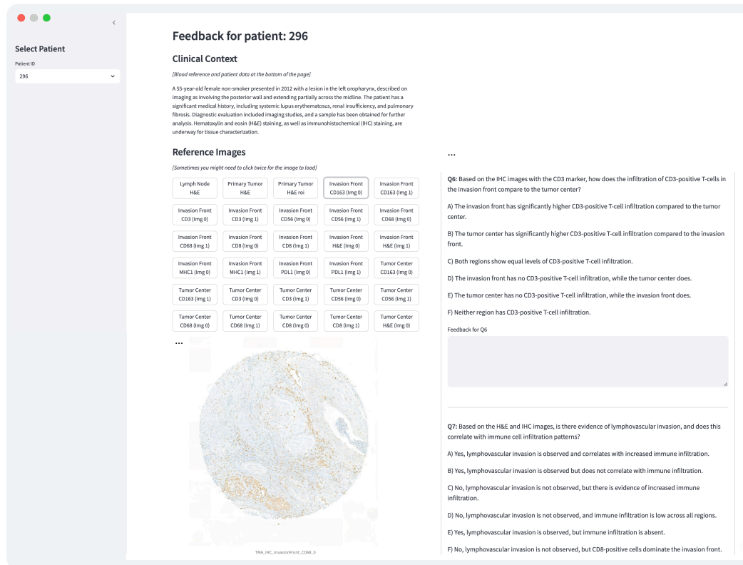
Figure 5: Companion app interface for clinical validation. The platform displays clinical context, reference images grouped by region and marker, and multiple-choice questions for expert review. Full-resolution slide viewers and inline feedback fields allow for efficient validation of benchmark items.
