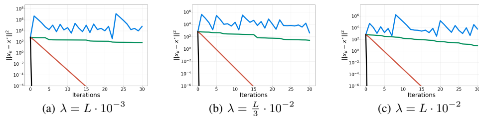
Figure 10: Ridge regression on mpg dataset; C(x) = \frac{2}{n} A^\top A .
