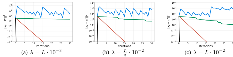
Figure 9: Ridge regression on housing dataset; C(x) = \frac{2}{n} A^\top A .
