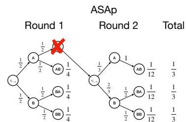
Figure 2: The probability mass of AA is distributed evenly.
