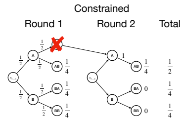
Figure 1: The entire probability mass of AA is shifted to AB.
