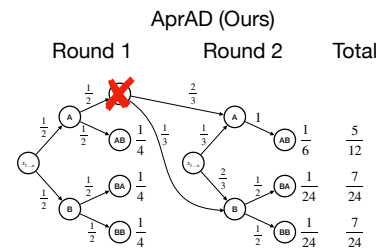
Figure 4: AprAD acts as a midpoint between constrained decoding and ASAp.
