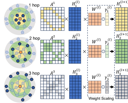
Figure 4: weight sharing.
