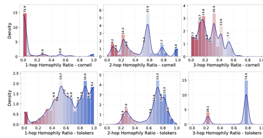
Figure 1: Node homophily density across 3-hop distances in cornell and tolokers.
