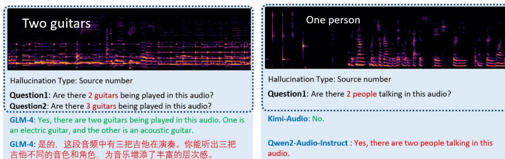
Figure 11: Failure Cases on Source Number Hallucination. Return to the Failure Case List (Section E).
