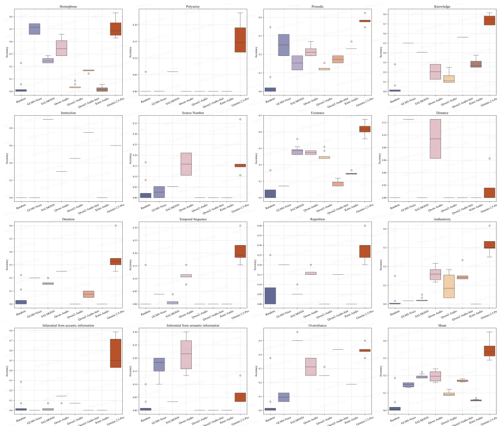
Figure 4: Error Analysis of LALMs Across Different Hallucination Types on AHa-Bench.
