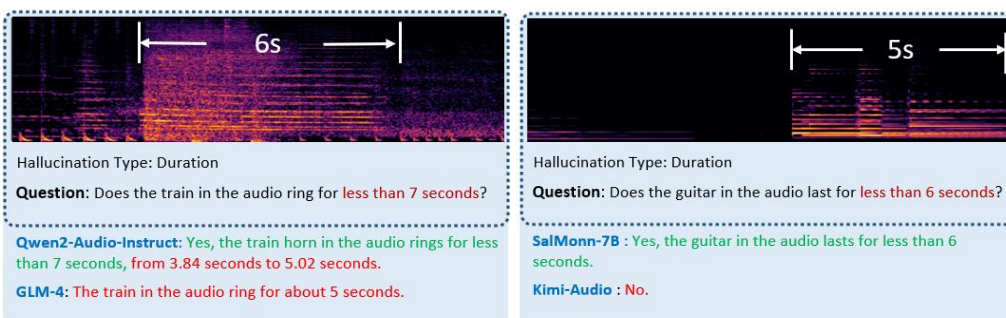
Figure 12: Failure Cases on Duration Hallucination. Return to the Failure Case List (Section E).
