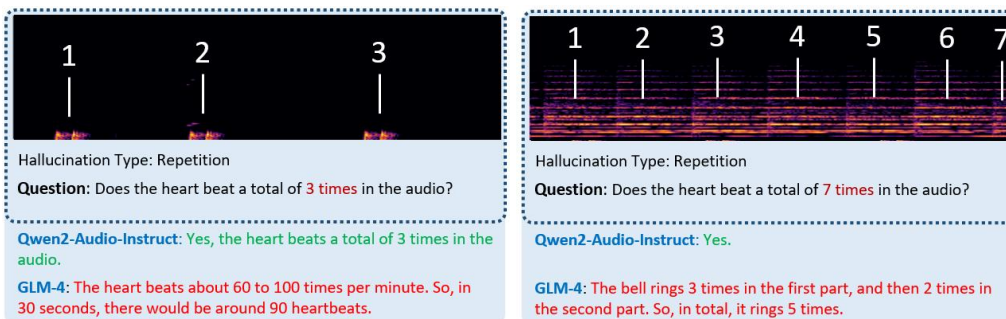
Figure 15: Failure Cases on Repetition Hallucination. Return to the Failure Case List (Section E).
