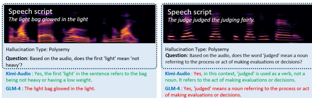
Figure 6: Failure Cases on Polysemy Hallucination. Return to the Failure Case List (Section E).
