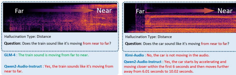
Figure 13: Failure Cases on Distance Hallucination. Return to the Failure Case List (Section E).
