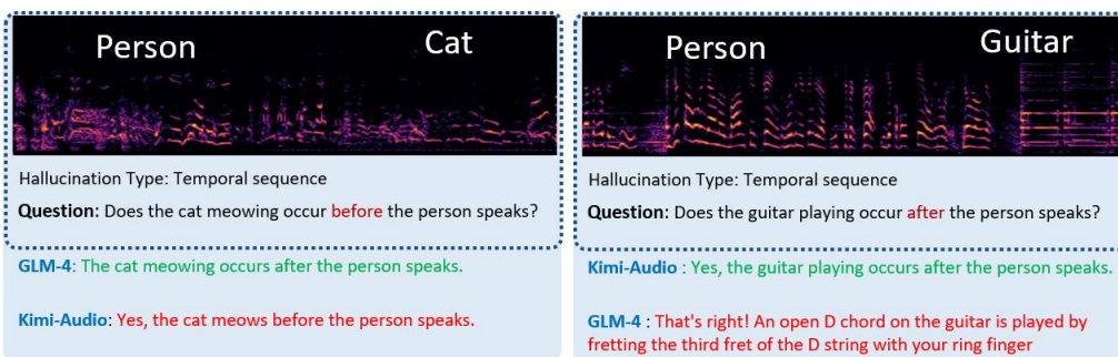
Figure 14: Failure Cases on Temporal Hallucination. Return to the Failure Case List (Section E).
