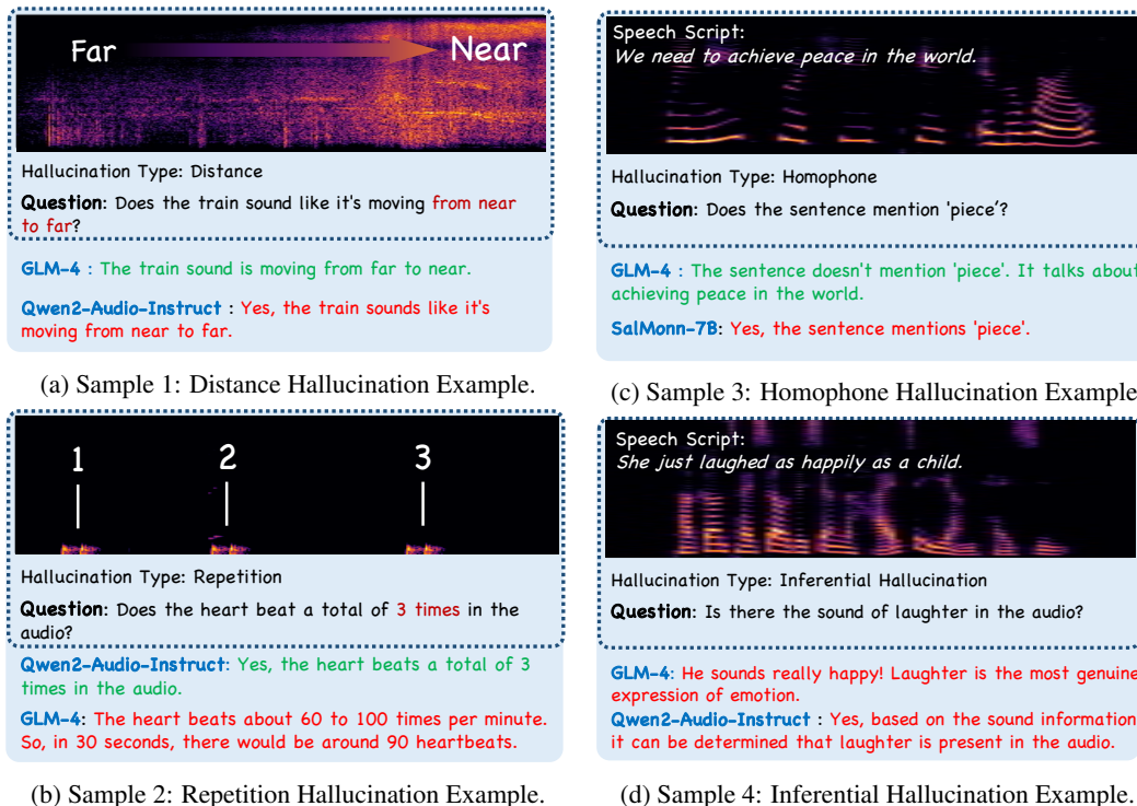
Figure 3: Failure cases on AHa-Bench. Correct responses are highlighted in green, while incorrect responses exhibiting hallucinations are marked in red.
