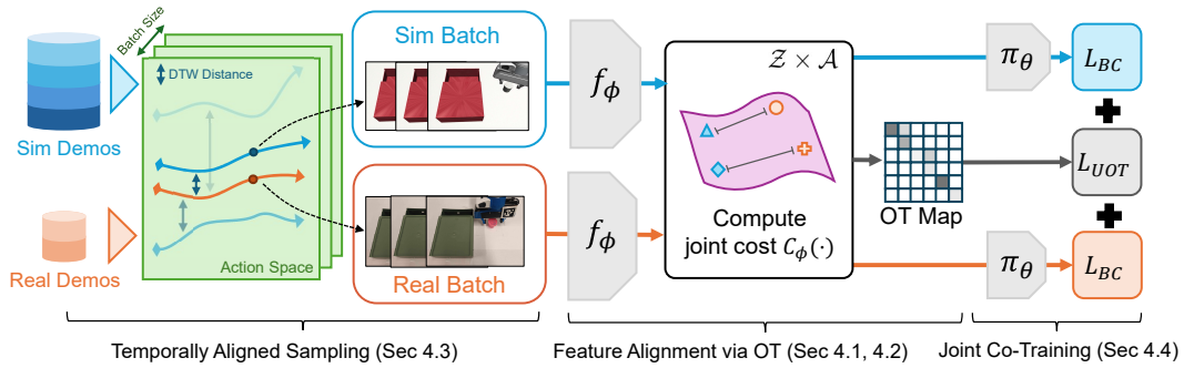
Figure 2: Method Overview. Our sim-and-real co-training framework learns a domain-invariant latent space to improve real-world performance using abundant simulation demos and a small number of real-world demos. It leverages an Unbalanced Optimal Transport loss and a temporal sampling strategy to address data imbalance and improve alignment quality during mini-batch training.
