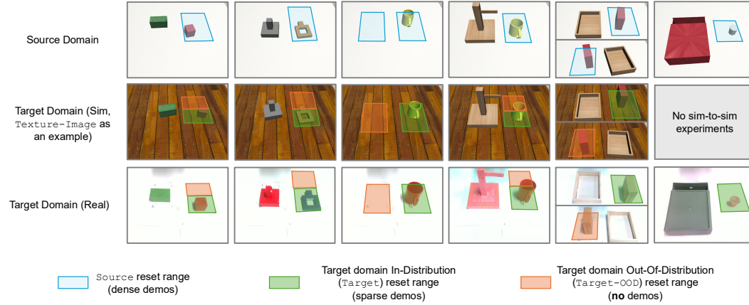
Figure 7: Reset Ranges for Each Task. The first row illustrates the Source region, where dense source-domain demonstrations are collected. The second row shows the Target and Target-00D reset ranges used in sim-to-sim transfer experiments. In this setting, the Target region is sparsely covered by demonstrations, while the Target-00D region contains no demonstrations and is used exclusively for policy evaluation. The third row similarly presents the Target and Target-00D regions for sim-to-real transfer experiments.
