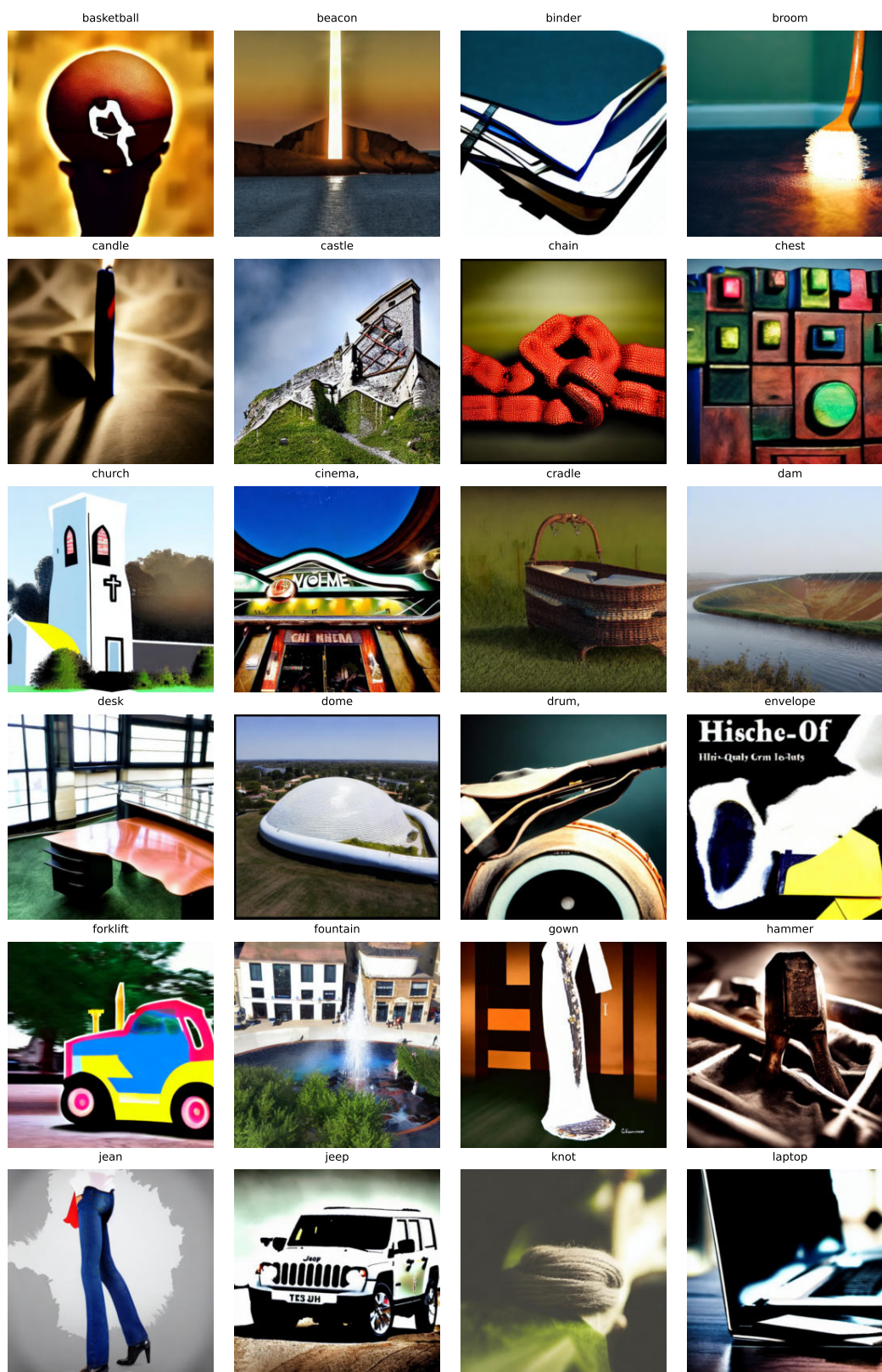
Figure 15: OOD samples generated by GOOD img on ImageNet, guided by low image likelihood (free energy). One sample per class is shown.
