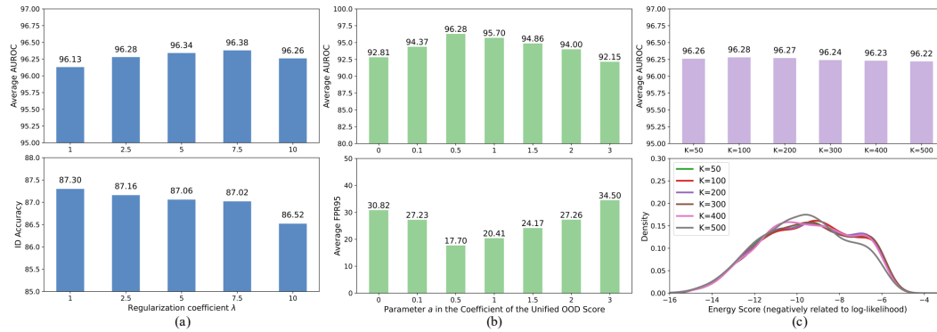
Figure 6: Ablation studies on key hyperparameters: (a) regularization weight \lambda in the OOD loss \mathcal{L}_{\text{ood}} ; (b) interpolation coefficient a in the unified OOD score (Eq. 8); (c) number of nearest neighbors K used in the KNN distance—top: for OOD scoring, bottom: for the sampling process.
