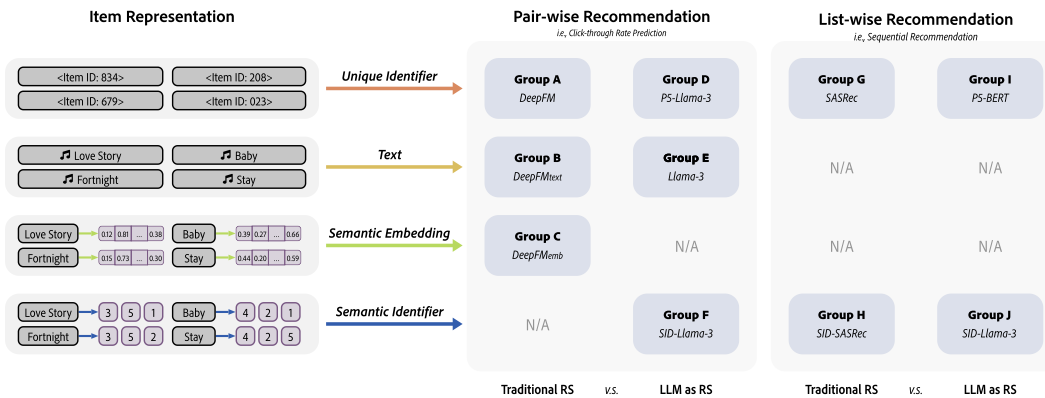
Figure 2: (Left) Various forms of item representations. (Right) Groups chosen for benchmarking and their representative methods. N/A: there is no or few related work, and it will not be evaluated.
