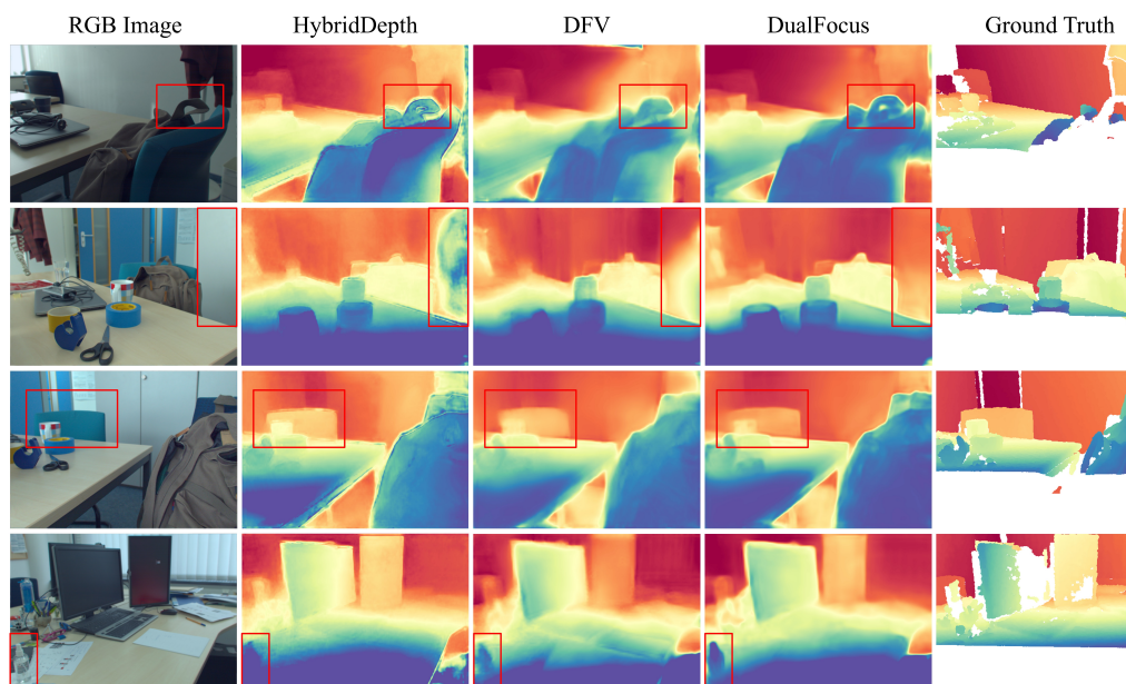
Figure 9: Qualitative comparison on the DDFF 12-Scene dataset.
