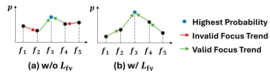
Figure 3: Our focal variational constraints ensure plausible focus probability distribution, reflecting natural focus transitions across the focal stack.
