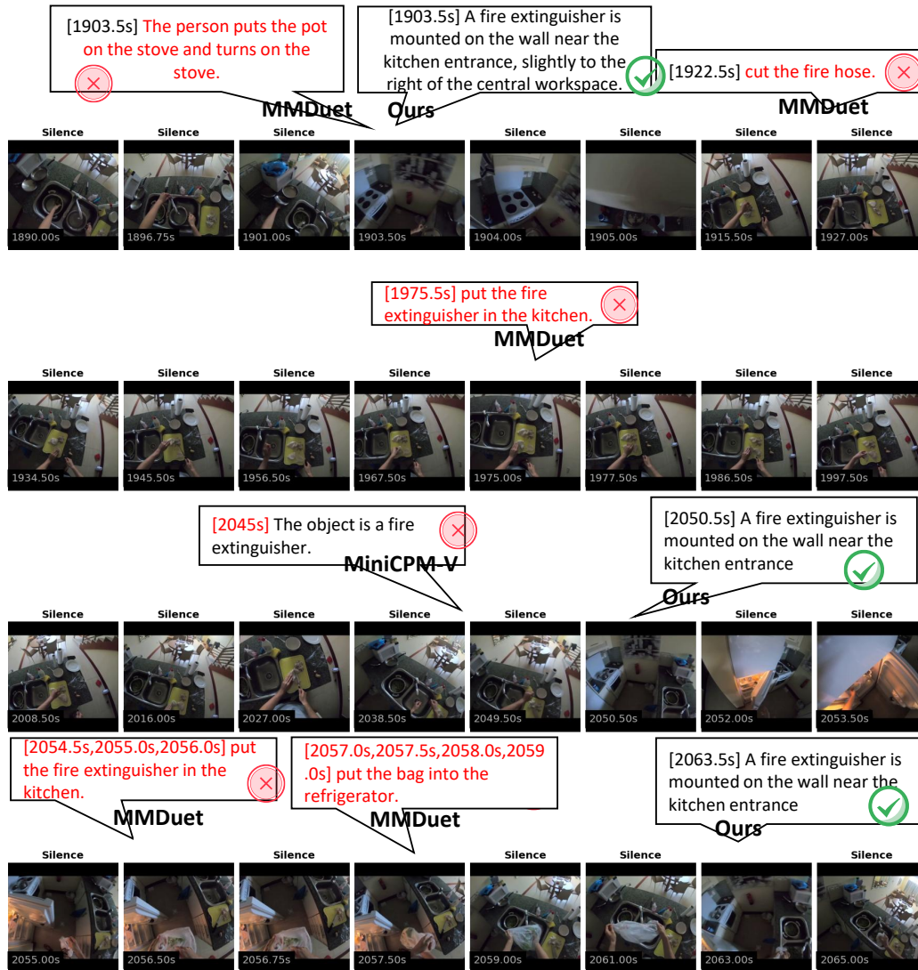
Figure 19: Qualitative Comparison with Baseline.
