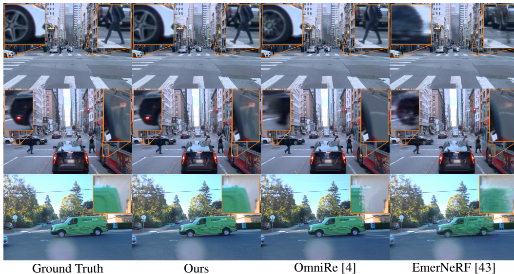
Figure 2: Visual quality comparisons (sequences s-952, 344, 975) show that our method achieves higher fidelity by producing way fewer artifacts on rapid motion (e.g., spinning wheels, edges), significantly reducing motion blur, and preserving finer details like reflections.
