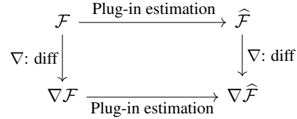
Figure 1: A commutative diagram illustrating that plug-in statistical estimation and differentiation can be interchanged for \mathcal{F} and \hat{\mathcal{F}} resulting in a single gradient estimator.
