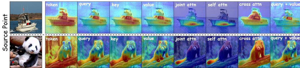
Figure 6: Visualization of matching probability maps using different MM-DiT facets. Features from query and value concentrate more precisely to the desired object parts.
