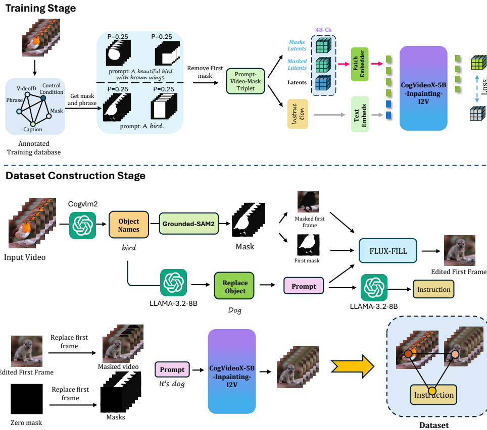
Figure 11: The training pipeline of our inpainter. Our inpainter employs a first-frame guided training strategy, where we randomly sample a mask from four different types during training. The input to DiT’s patch embedder concatenates the noisy latents, masks latents, and masked latents into a 3c \times f \times h \times w tensor. In training, the first frame of the masked video is taken directly from the original video, and the rest are holed frames. The first frame of masks is all zeros and the rest are holed masks. During inference, the first frame of the masked video is replaced by a Flux-Fill-inpainted image, the first frame of masks are all zeros, and subsequent frames use dilated holed masks.
