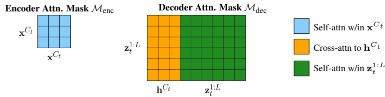
Figure 4: Example attention masks used in training full-sequence diffusion with an encoder-decoder architecture, for L = 6 tokens. We denote clean tokens in \mathbf{z}_t^{1:L} as \mathbf{x}^{C_t} , where C_t corresponds to their token indices. In this example, |C_t| = 3 . Left: The encoder mask \mathcal{M}_{\text{Enc}} \in \{0, 1\}^{|C_t| \times |C_t|} enables clean tokens to attend to other clean tokens in the sequence. Right: The decoder mask \mathcal{M}_{\text{Dec}} \in \{0, 1\}^{L \times (L + |C_t|)} uses bidirectional attention across the noised sequence \mathbf{z}_t^{1:L} and cross-attention to the encoder’s output representation \mathbf{h}^{C_t} .
