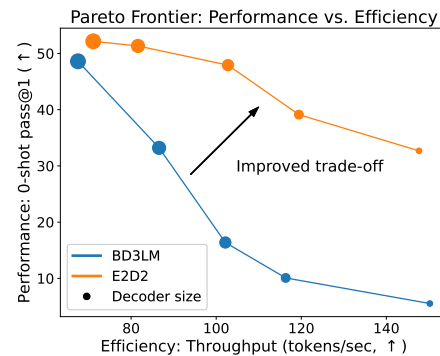
Figure 3: Mapping the Pareto Frontier: Larger models increase accuracy on GSM8K at the cost of slower decoding. E2D2 improves this trade-off.
