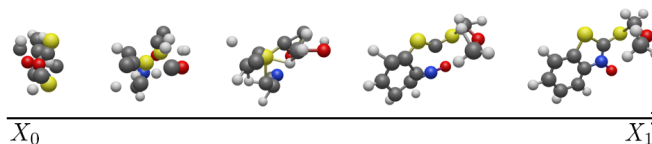
Figure 6: Example of ASBS generative process on amortized conformer generation. Given an unseen molecular topology g \in \mathcal{G}_{\text{test}} from the test set—C0CSc1sc2ccccc2[n+]1[0-] in this case—ASBS transports samples from the harmonic prior X_0 \sim \mu_{\text{harmonic}} to generate conformers X_1 .
