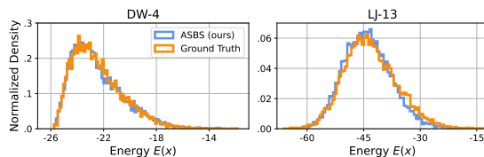
Figure 3: The energy histograms of DW-4 and LJ-13 from Table 2. ASBS generates samples whose energy profiles closely match those of the ground-truth samples.
